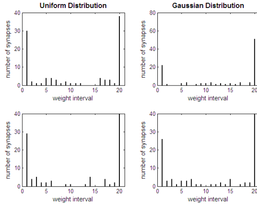
Fig. 2: Bimodal distribution of the excitatory synaptic weight distribution of a single excitatory neuron after STDP mediated simulation in an Izhikevich network. Left column (initially uniform weight distribution) has two plots showing the dynamic bimodal distributions of excitatory synaptic weights after 100 (upper) and 120 (lower) seconds of simulation time. Right column (initially Gaussian weight distribution) shows a dynamic bimodal distribution as well, after simulation time of 120 (upper) and 130 (lower) seconds, respectively. In actual, we can see the network can reach dynamic stability by using two time spans in both distributions. The X-axis shows the bin index and the Y-axis shows the number of synapses in a certain bin.
