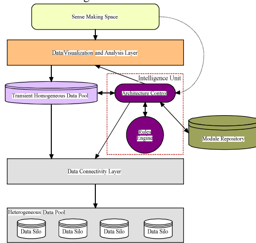
Figure 4: INVISQUE Architecture
