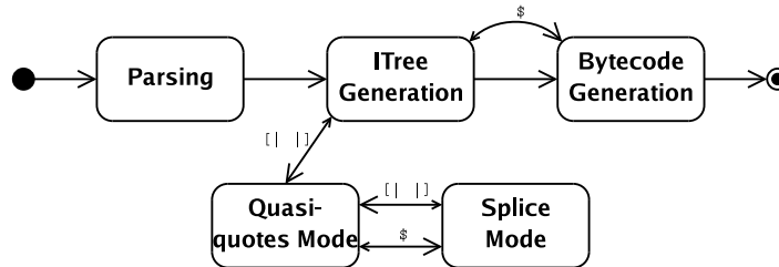
Fig. 1. Converge compiler states.
