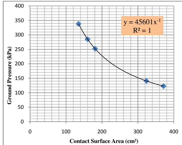
Fig. 11. Test results showing how the contact surface area affects the ground pressure.
