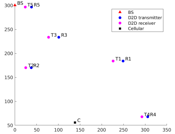
Fig. 2. A typical example of simulation model for a D2D underlying cellular network consisting of a BS, a CU, and 5 pairs of D2D users within an area of 300 m \times 300 m.
