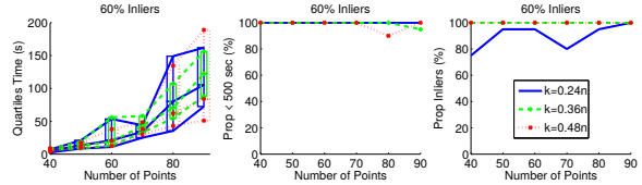
Figure 4: Results of BnB for increasing number of points and 60% inliers, across different values of k .
