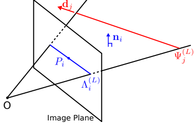
Figure 1: An illustration of the terminology used in defining a distance measure for lines. \Lambda_i^{(L)} denotes a 2D line, P_i its midpoint and \mathbf{n}_i the normal to its backprojected plane. \Psi_j^{(L)} denotes a 3D line and \mathbf{d}_j its normalised direction vector.
