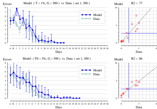
Figure 6: Static noise model (top) and dynamic noise model (bottom) compared with the data (Yerkes and Dodson, 1908). The dynamic model achieves the better match.
