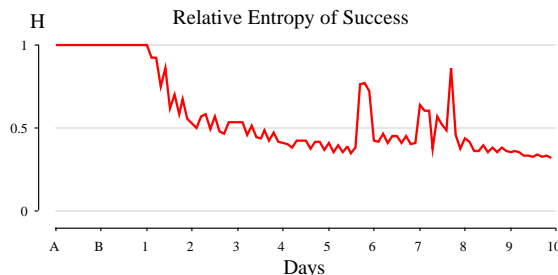
Figure 3: Relative entropy of success of the choice rules. Entropy increases on errors (see Figure 1) and when new rules are learned.
